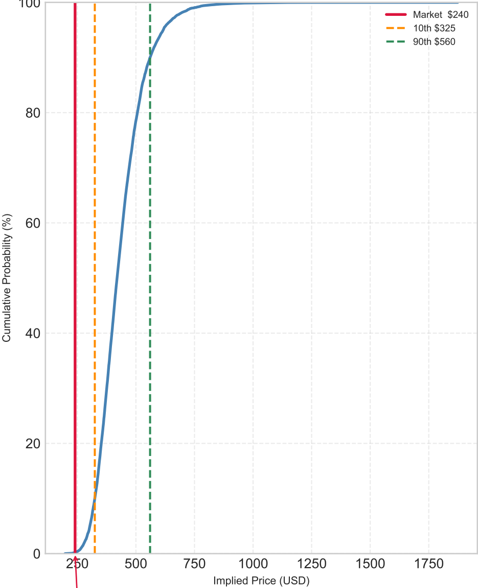
Cumulative Distribution
